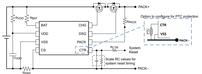
Simplified Schematic
