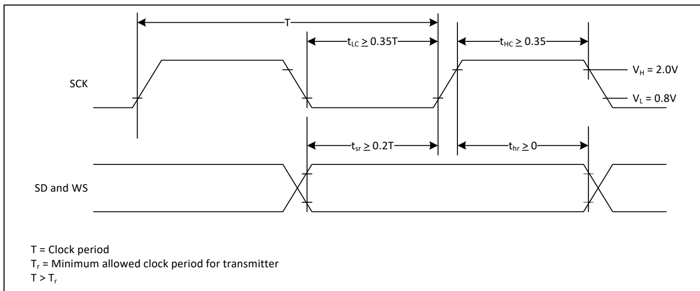
Figure 28. I 2 S Receiver Timing
