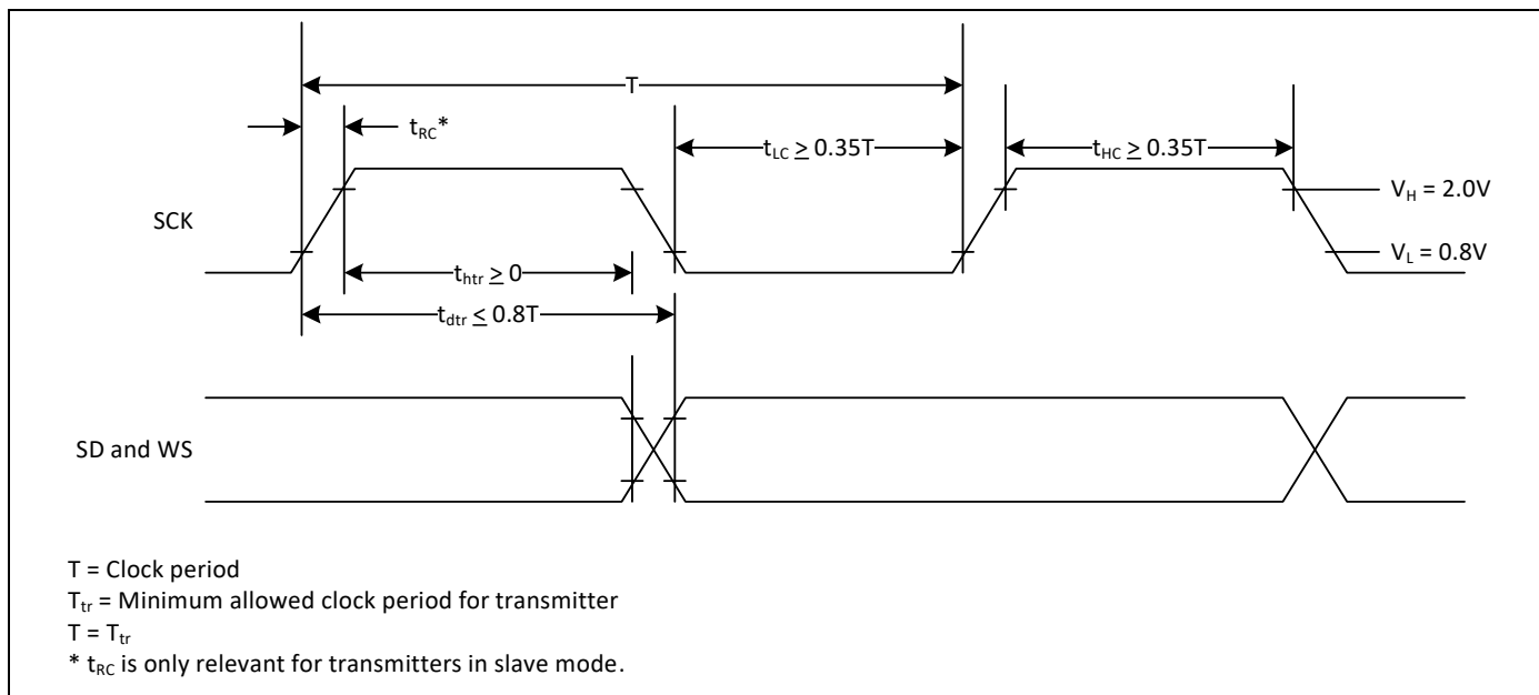
Figure 27. I 2 S Transmitter Timing
