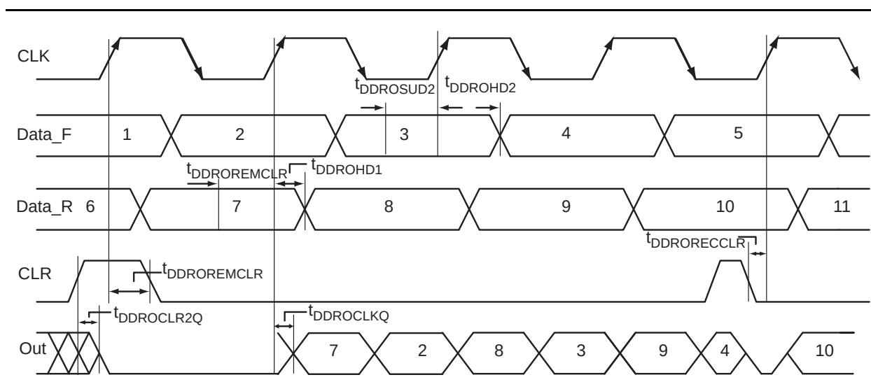
Figure 2-20 • Output DDR Timing Diagram
