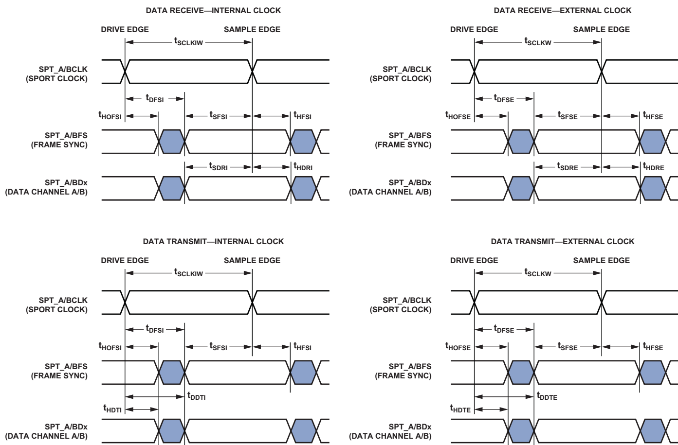
Figure 36. Serial Ports
