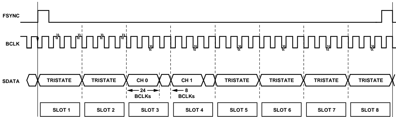
Figure 15. TDM-8, BCLK = 256 \times f_s , CONFIG Pin Open
