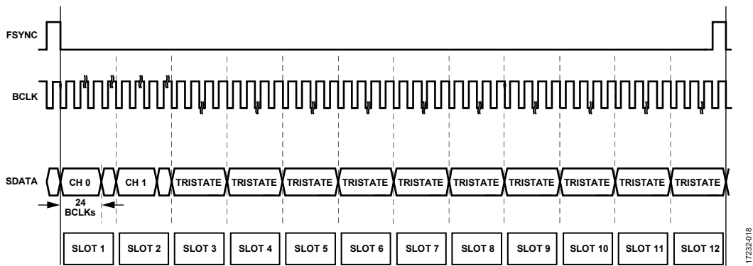
Figure 18. TDM-12, BCLK = 384 \times f_s , CONFIG Pin Tied to GND
