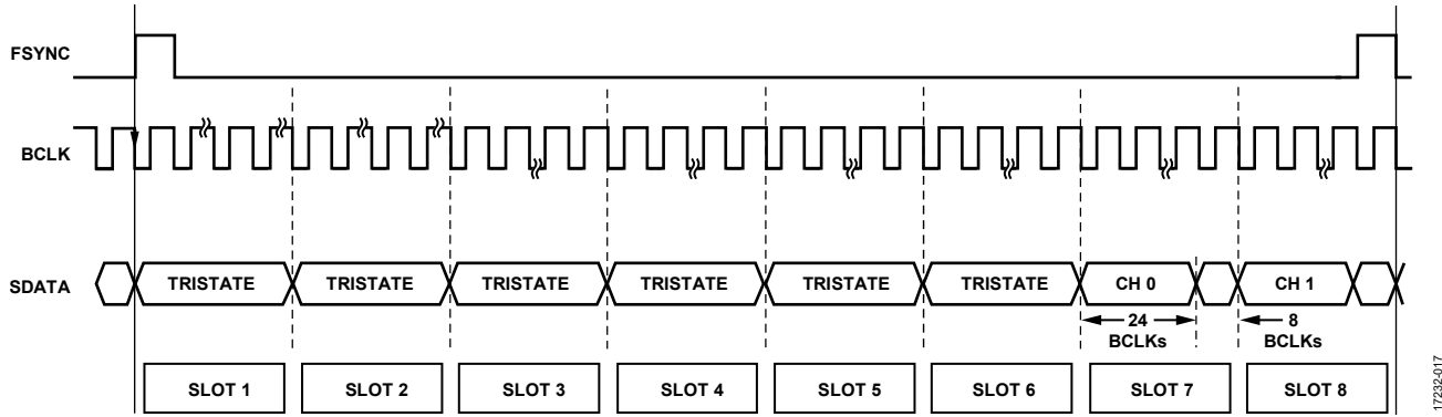
Figure 17. TDM-8, BCLK = 256 \times f_s , CONFIG Pin Tied to GND Through a 47 k \Omega Resistor
