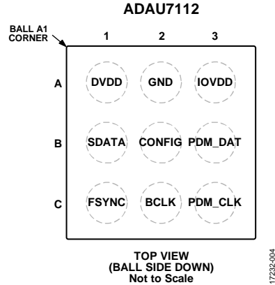
Figure 4. Pin Configuration
