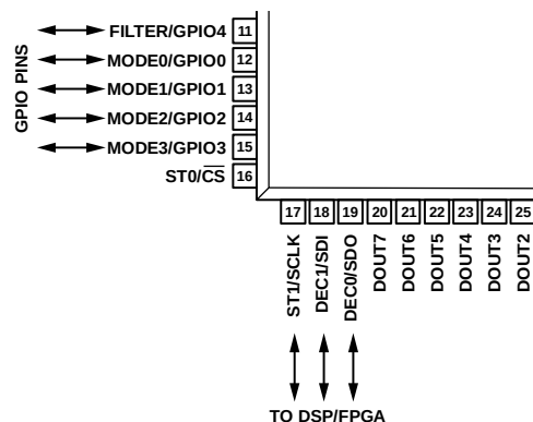
Figure 82. GPIO Functionality
