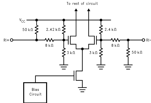
Figure 8. Typical Receiver Input Circuit
