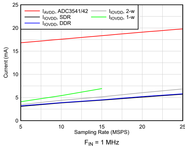
F_{IN} = 1 \text{ MHz} Figure 6-15. Current vs Sampling Rate
