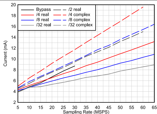
F_{IN} = 5 MHz, 2-w serial CMOS Figure 6-61. I_{OVDD} Current vs Decimation
