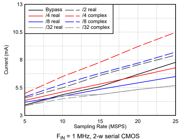
F_{IN} = 1 \text{ MHz} , 2-w serial CMOS Figure 6-16. I_{OVDD} Current vs Decimation
