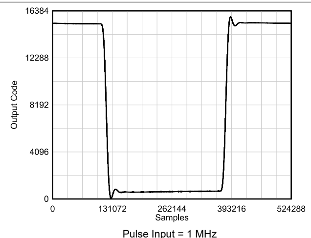
Figure 6-35. Pulse Response
