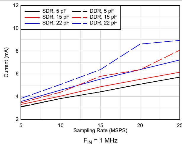
F_{IN} = 1 \text{ MHz} Figure 6-17. I_{OVDD} Current vs Output Load
