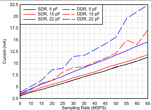
F_{IN} = 5 MHz, DDC Bypass Figure 6-63. I_{OVDD} Current vs Output Load
