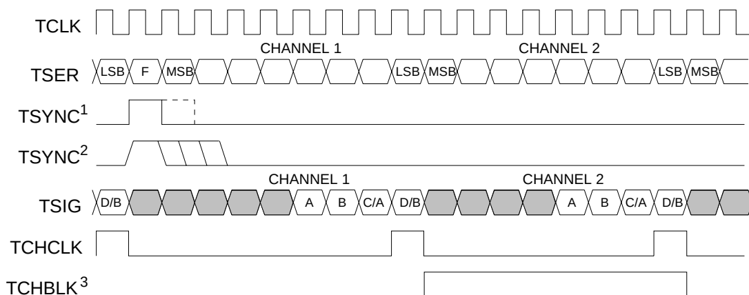
Figure 10-10. T1 Transmit-Side Boundary Timing (Elastic Store Disabled)
