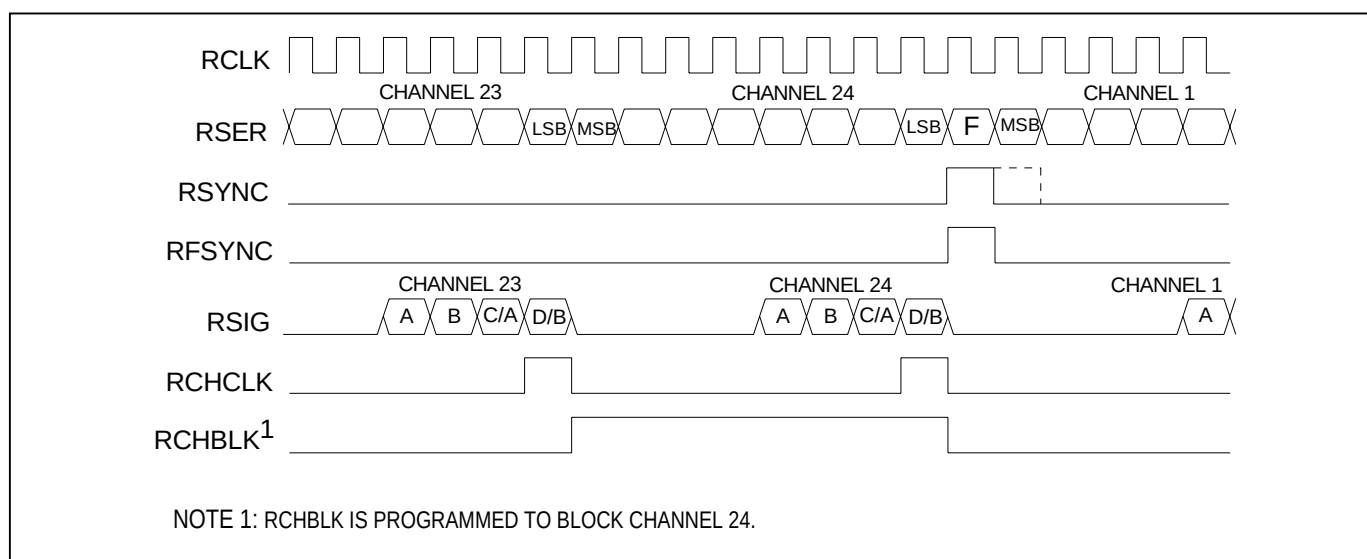
Figure 10-3. T1 Receive-Side Boundary Timing (Elastic Store Disabled)
