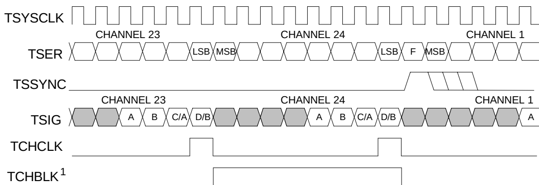
Figure 10-11. T1 Transmit-Side 1.544MHz Boundary Timing (Elastic Store Enabled)
