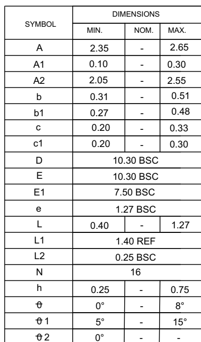
Figure 40 SOIC 16-lead, 300-mil body width (SO3016)
