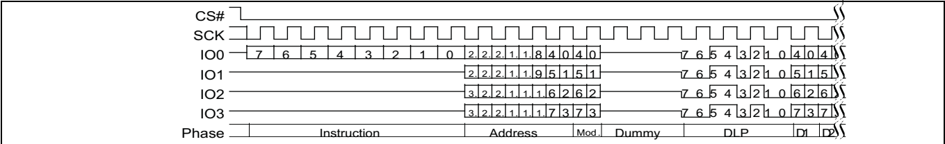
Figure 96 DDR quad I/O read initial access (4-byte address, EEh or EDh [ExtAdd = 1], EHPLC = 01b) [48]
