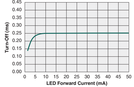
Typical Turn-Off vs. LED Forward Current ( I_L=1A_{DC}, T_A=25^\circ\text{C} )
