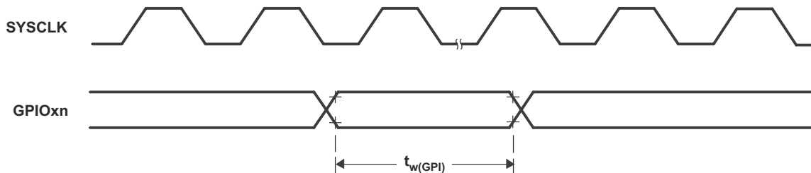
Figure 7-32. General-Purpose Input Timing
