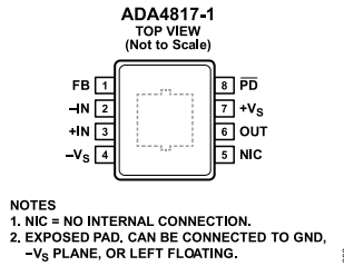
Figure 6. ADA4817-1 Pin Configuration (8-Lead SOIC)
