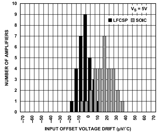
Figure 42. Input Offset Voltage Drift Histogram ( V_S = 5V )
