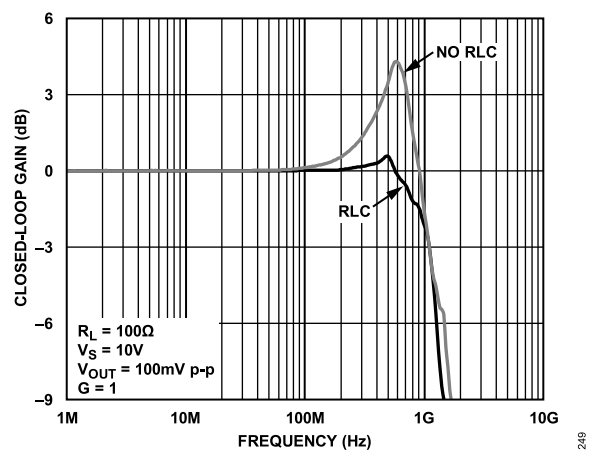
Figure 62. Frequency Response with RLC Circuit
