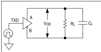
Figure 2. Driver Timing Test Circuit
