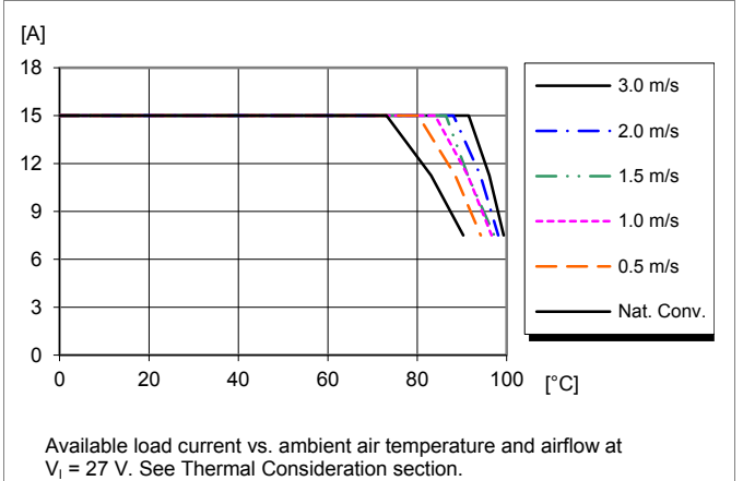
Output Current Derating, Vin=27V, test board 2
