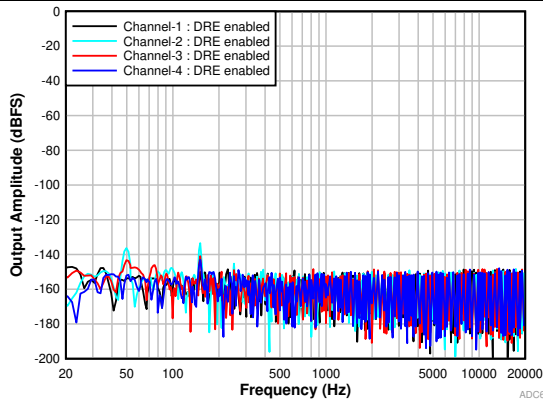
Figure 8. FFT With Idle Input With DRE Enabled
