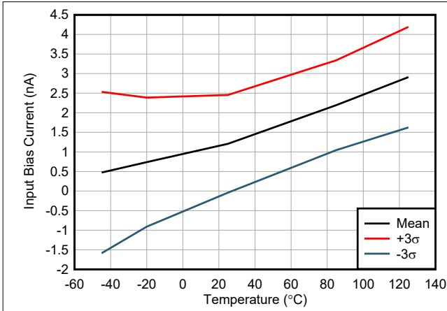
Figure 7-13. Input Bias Current vs Temperature
