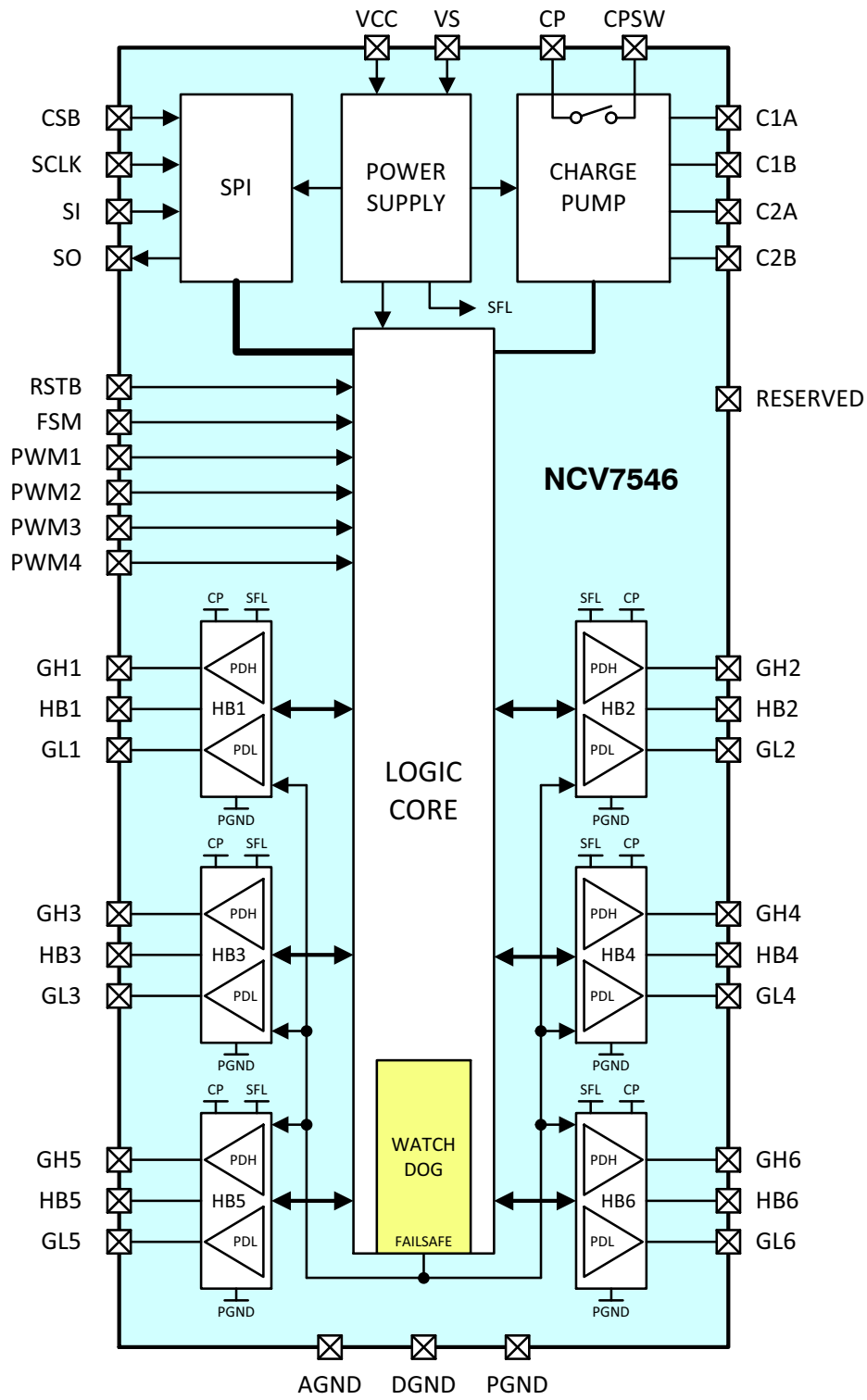
Figure 1. Block Diagram
