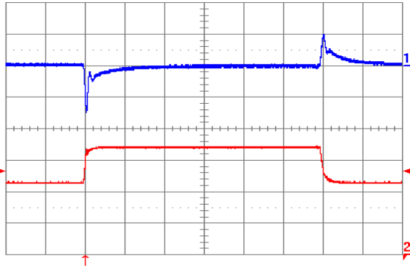
Fig. 2.0V.9: Output voltage response to load current step-change (22.5 A – 33.75 A – 22.5 A) at V_{in} = 48\text{ V} . Top trace: output voltage (100 mV/div.). Bottom trace: load current (10 A/div). Current slew rate: 1 A/ \mu\text{s} . C_o = 470\text{ }\mu\text{F} tantalum + 1 \mu\text{F} ceramic. Time scale: 0.2 ms/div.
