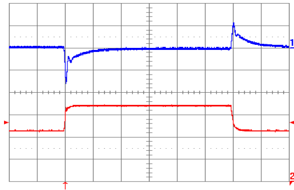
Fig. 1.8V.9: Output voltage response to load current step-change (22.5 A – 33.75 A – 22.5 A) at V_{in} = 48 V. Top trace: output voltage (20 mV/div.). Bottom trace: load current (10 A/div). Current slew rate: 1 A/ \mu s. C_o = 470 \mu F tantalum + 1 \mu F ceramic. Time scale: 0.2 ms/div.
