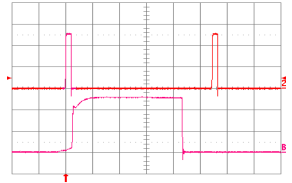
Fig. 1.5V.15: Load current (top trace, 20\ \text{A}/\text{div} , 20\ \text{ms}/\text{div} ) into a 10\ \text{m}\Omega short circuit during restart, at V_{in} = 48\ \text{V} . Bottom trace ( 20\ \text{A}/\text{div} , 1\ \text{ms}/\text{div} ) is an expansion of the on-time portion of the top trace.
