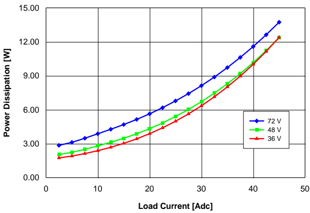
Fig. 1.8V.5: Power dissipation vs. load current and input voltage for converter mounted vertically with air flowing from pin 3 to pin 1 at a rate of 300 LFM (1.5 m/s) and T_a = 25\text{ }^\circ\text{C} .
