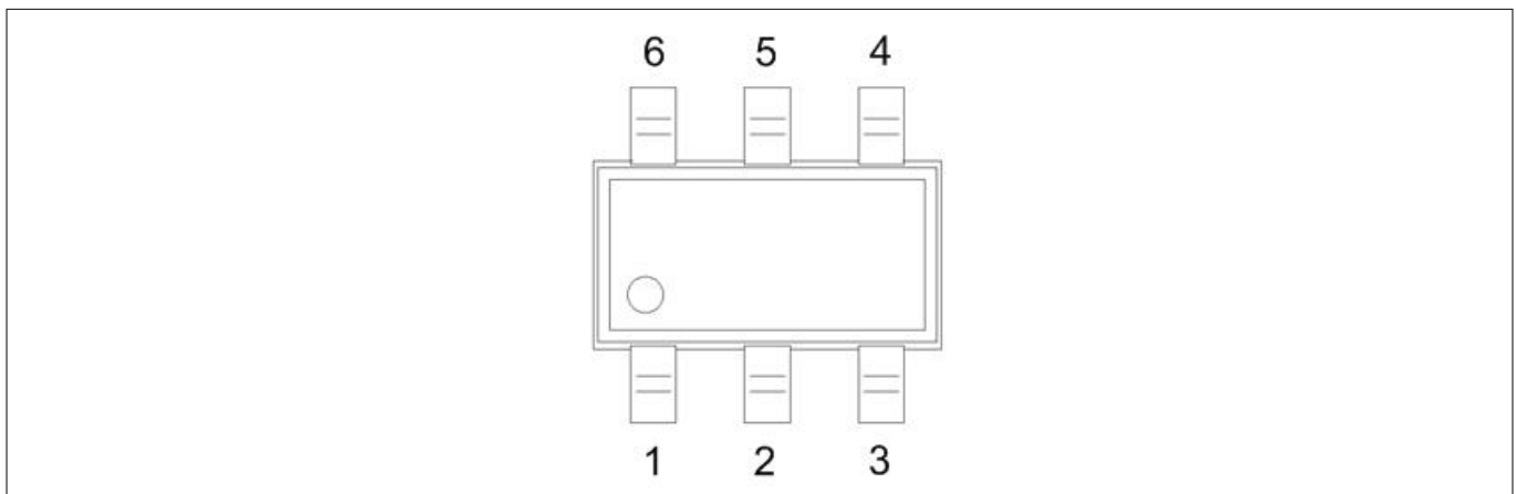
Figure 2 TLE493D-P2B6 pinout
