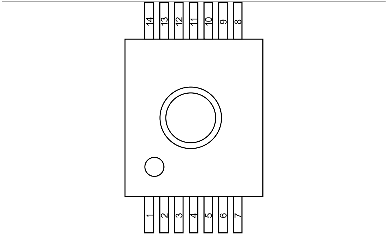
Figure 2 Pin Configuration
