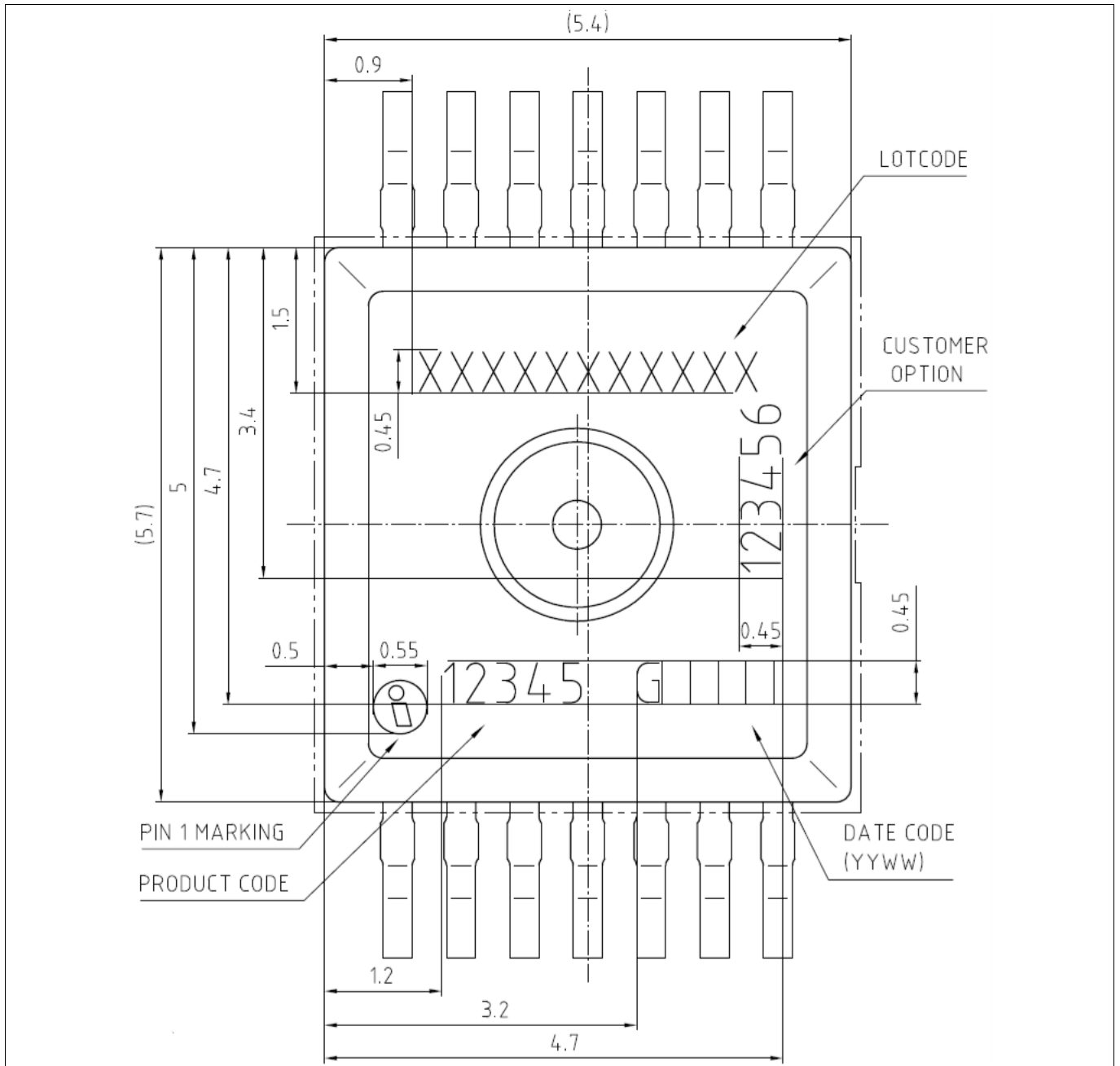
Figure 8-2 Marking information
