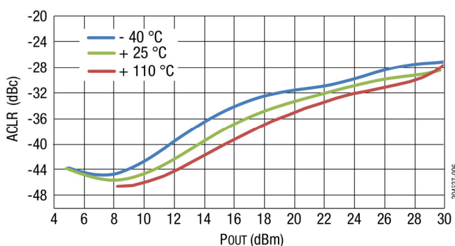
Figure 6. LTE 5x20 MHz ACLR1 vs Pout Across Temperature
