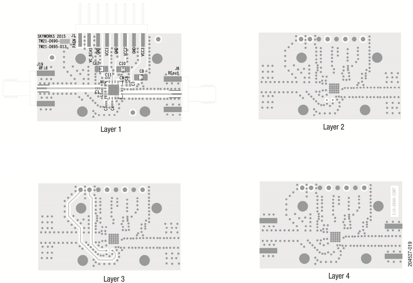
Figure 19. SKY66317-11 Board Layer Detail
