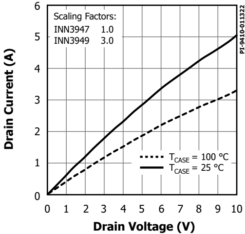
Figure 33. Output Characteristics.
