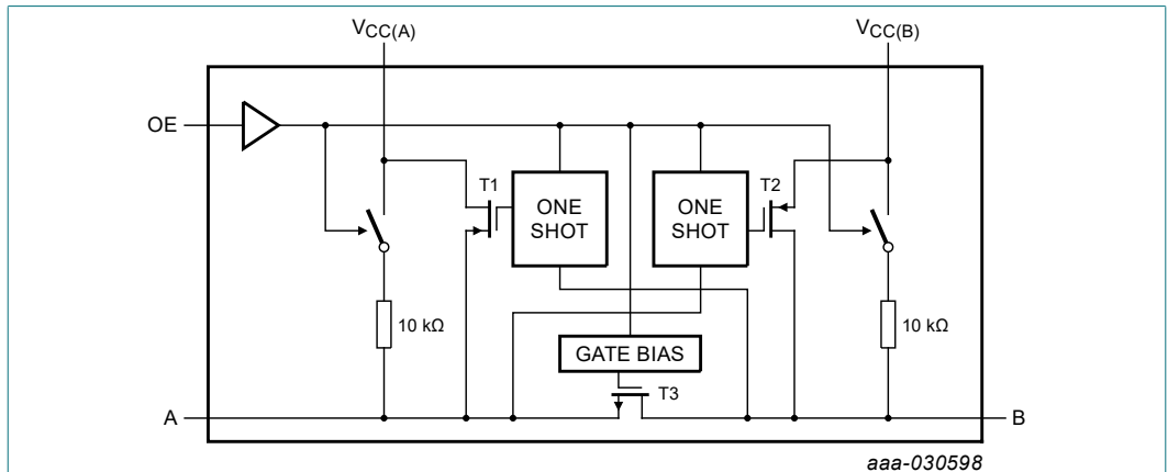
Fig. 7. Architecture of NXS0102-Q100 I/O cell (one channel)
