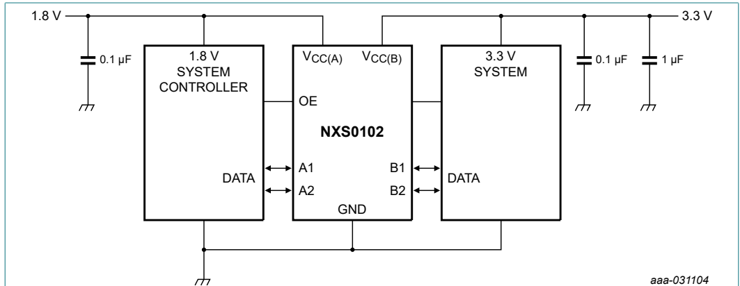
Fig. 6. Typical operating circuit
