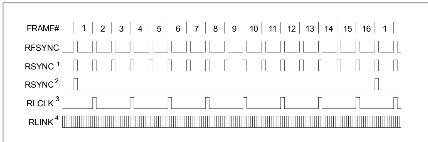
Figure 31-11. Receive-Side Timing
