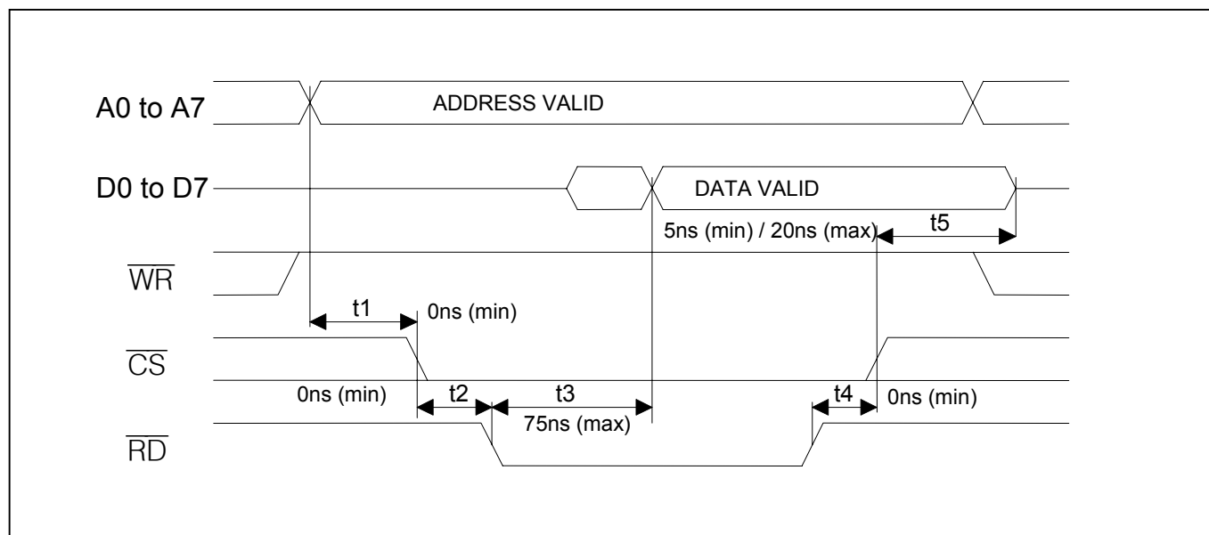
Figure 33-4. Intel Bus Read Timing (BTS = 0/MUX = 0)
