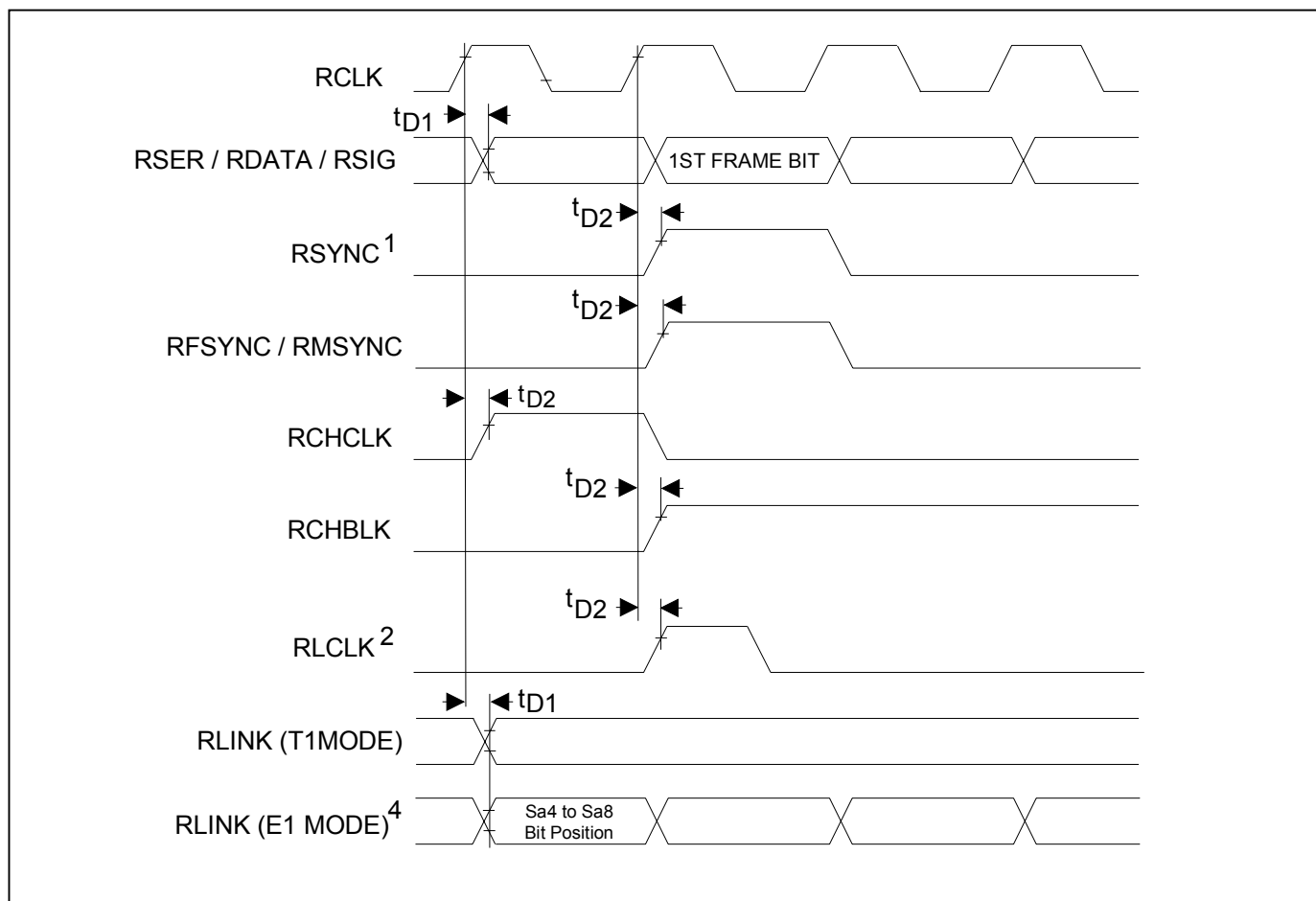
Figure 33-8. Receive-Side Timing
