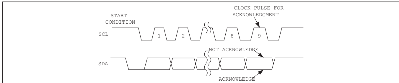
Figure 35. Acknowledge
