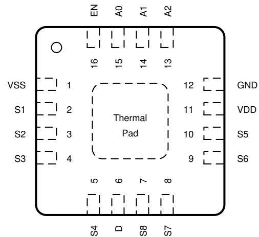
Figure 6-1. PW Package, 16-Pin TSSOP (Top View) Figure 6-2. RUM Package 16-Pin WQFN (Top View)
