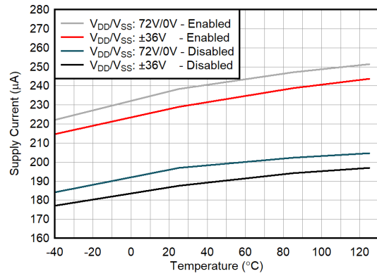
Figure 7-26. Supply Current vs Temperature
