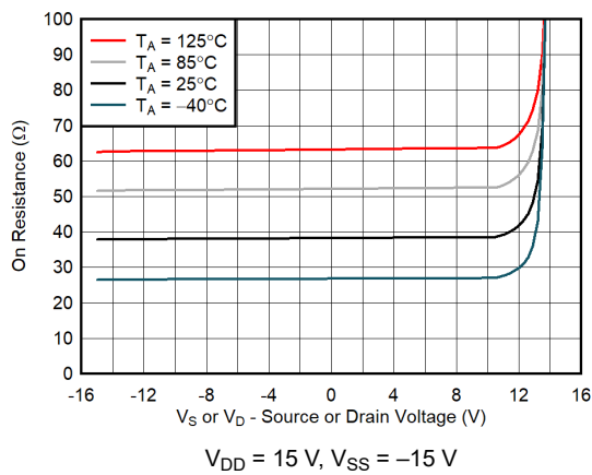
Figure 7-5. On-Resistance vs Source or Drain Voltage
