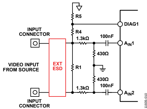
Figure 11. Diagnostic Connections
