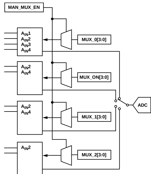
Figure 14. Manual Muxing Scheme for ADV7281 and ADV7282
