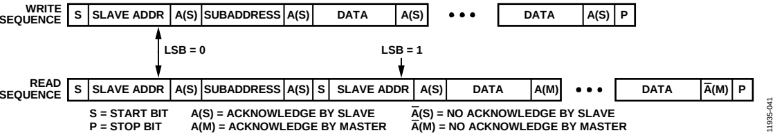
Figure 42. Read and Write Sequence
