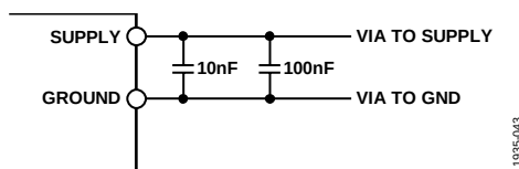
Figure 44. Recommended Power Supply Decoupling
