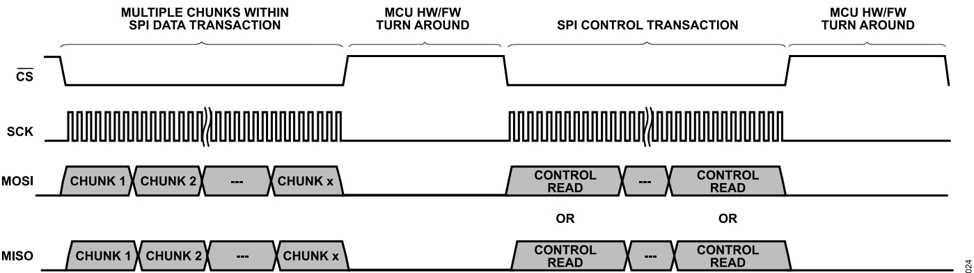
Figure 23. Ethernet Data Frame Transfer Followed by Control Transfer
