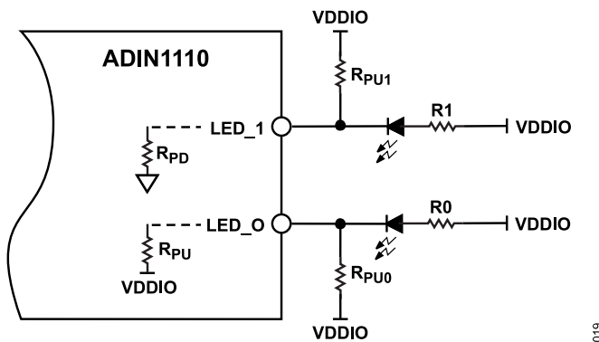
Figure 17. Recommended Active Low LED Circuit
