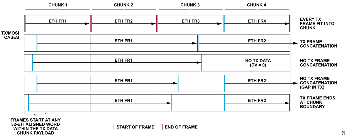
Figure 26. Transmit Data Chunk Cases
