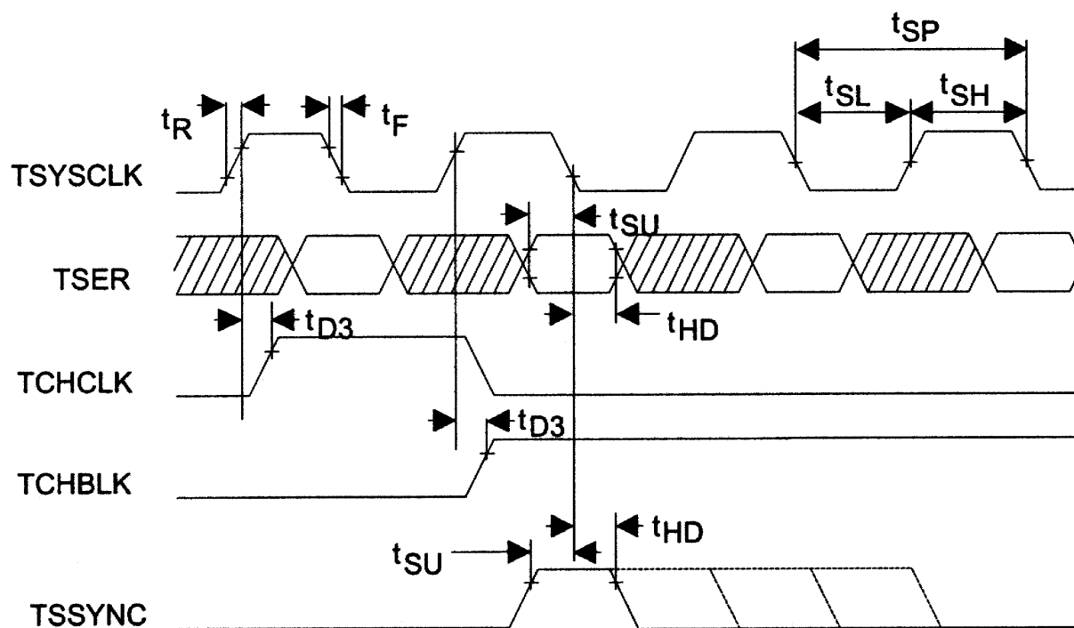
Figure 21-12. TRANSMIT SYSTEM SIDE AC TIMING
