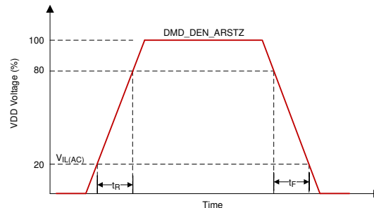
Figure 6-4. LPSDR Input Slew Rate
