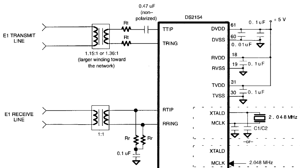
Figure 13-1. External Analog Connections
