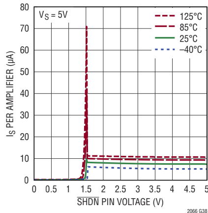
Supply Current vs \overline{SHDN} Pin Voltage
