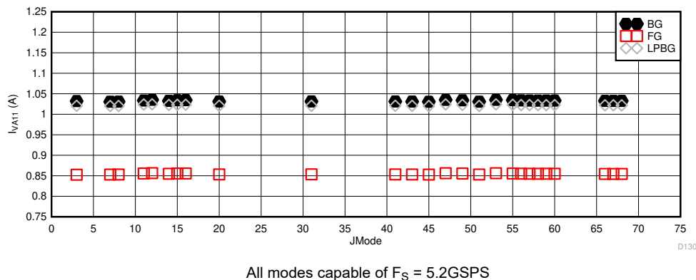
Figure 5-114. Dual Channel Mode: I_{V_{A11}} vs JMODE at 5.2GSPS
