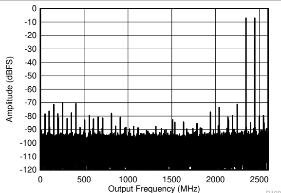
Figure 5-25. Dual Channel Mode: Two Tone FFT at 2397 MHz
