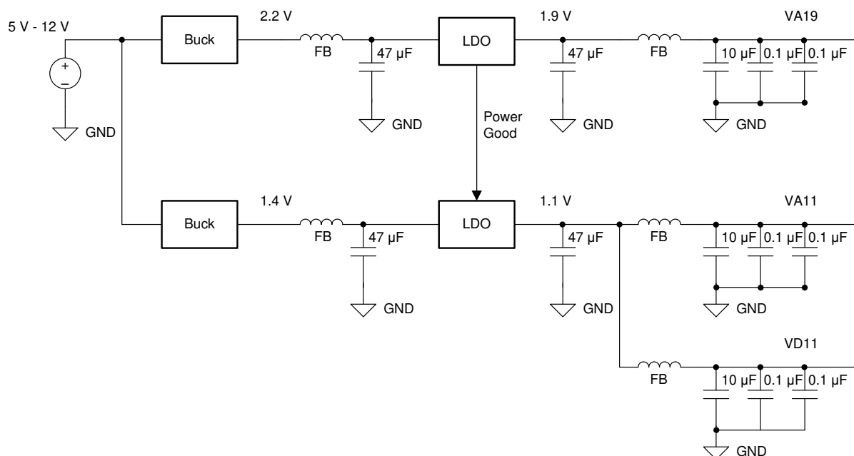
Figure 7-13. LDO Linear Regulator Approach Example
