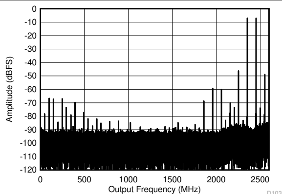
Figure 5-26. Dual Channel Mode: Two Tone FFT at 4197 MHz
