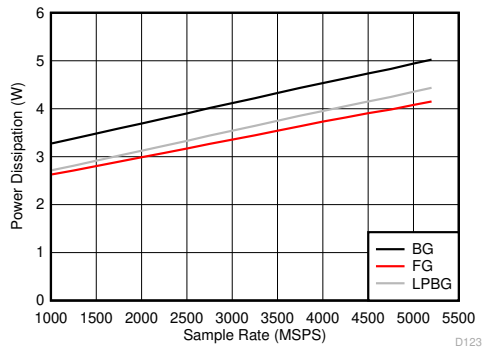
Figure 5-139. Dual Channel Mode: Power Dissipation vs Sample Rate
