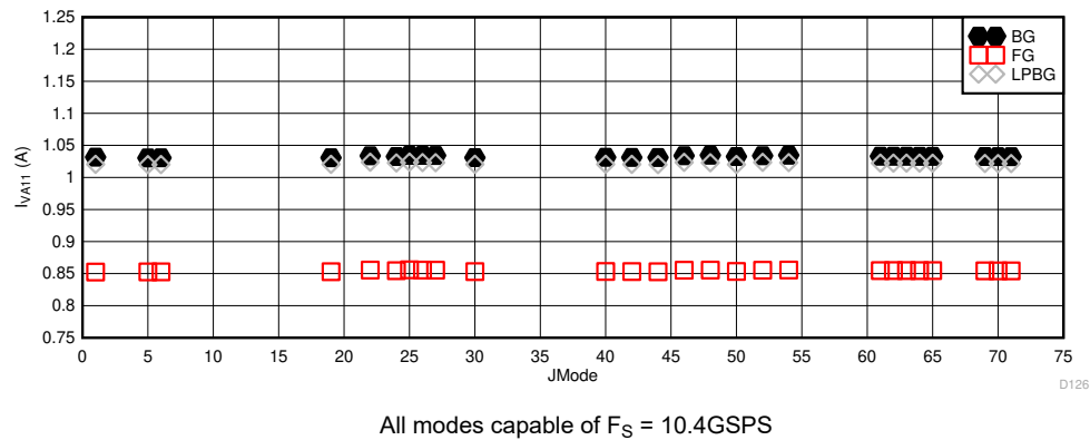
Figure 5-110. DES Mode: I_{VA11} vs JMODE at 10.4GSPS
