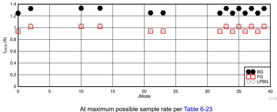
Figure 5-117. Other Modes with Lower Maximum F_S : I_{VA19} vs JMODE
