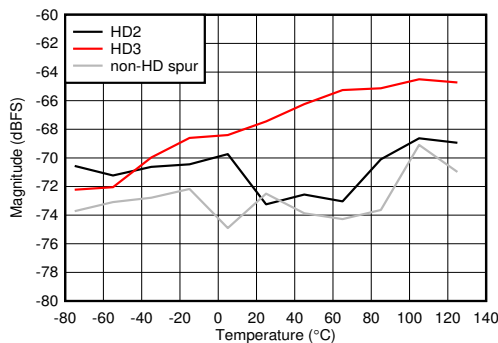
Figure 5-91. Dual Channel Mode: HD2, HD3 and Worst non-HD Spur vs Temperature
