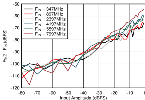
Figure 5-65. DES Mode: \text{Fs}/2 - F_{\text{IN}} vs Input Amplitude and Frequency
