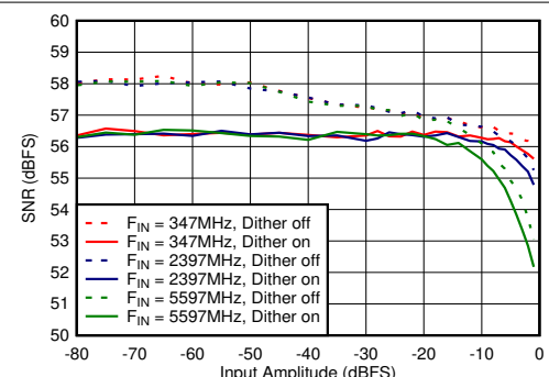
Figure 5-72. Dual Channel Mode: SNR vs Input Amplitude and Dither
