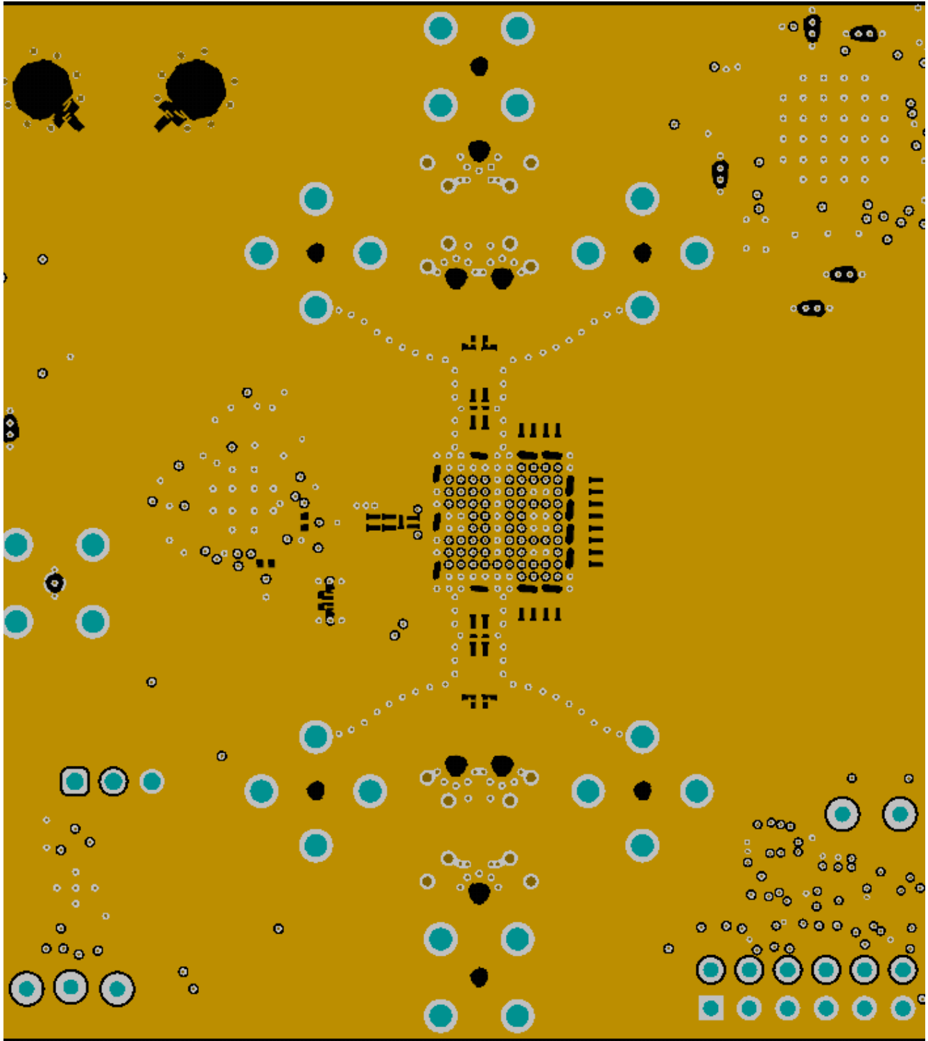
Figure 7-16. GND1 Cutouts to Optimize Impedance of Component Pads
