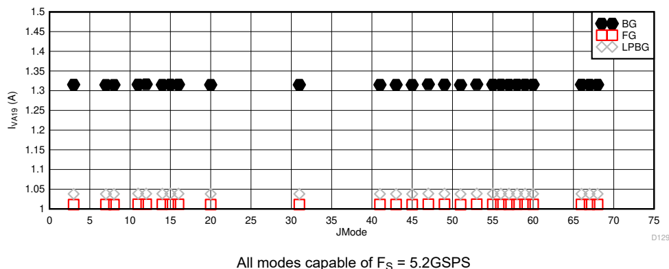
Figure 5-113. Dual Channel Mode: I_{V_{A19}} vs JMODE at 5.2GSPS
