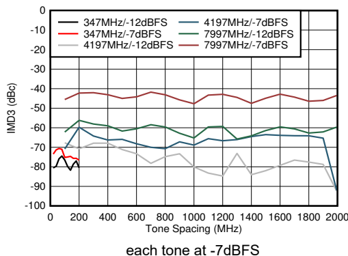
Figure 5-101. DES Mode: IMD3 vs Tone Spacing
