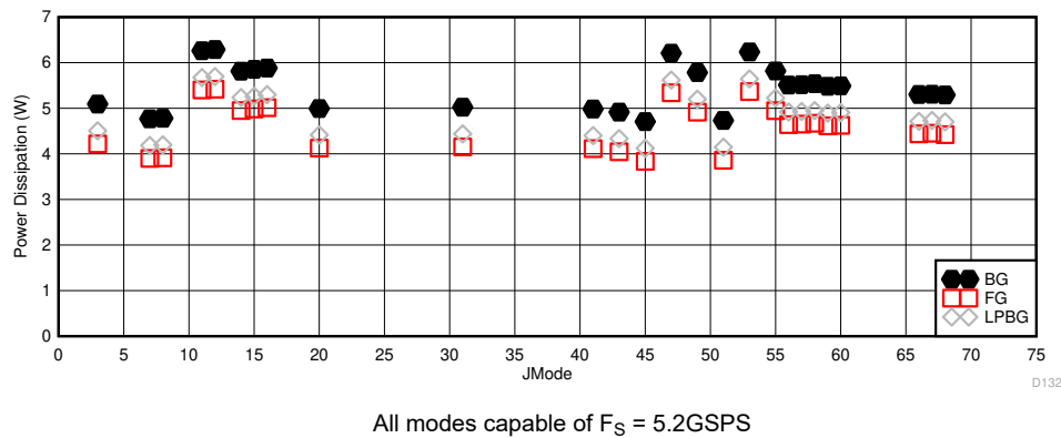
Figure 5-116. Dual Channel Mode: Power Dissipation vs JMODE at 5.2GSPS
