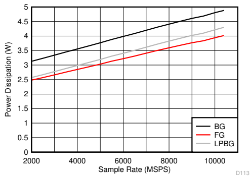
Figure 5-127. DES Mode: Power Dissipation vs Sample Rate
