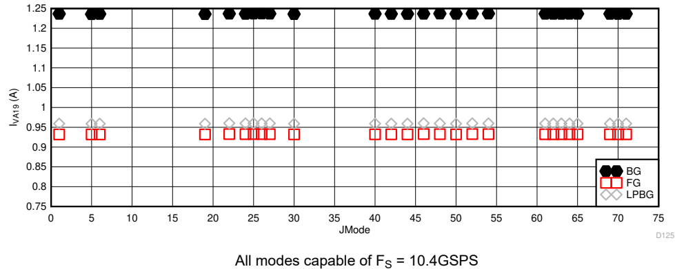
Figure 5-109. DES Mode: I_{VA19} vs JMODE at 10.4GSPS
