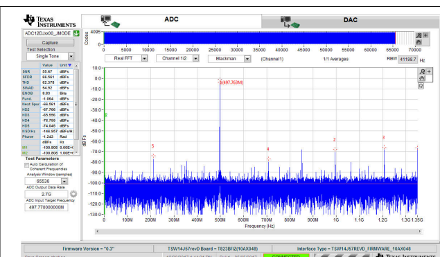
Figure 7-3. FFT for 497.77-MHz Input Signal, 2.7 GSPS, JMODE2
