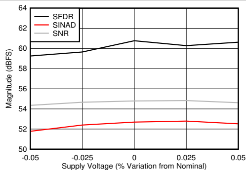
Figure 5-93. DES Mode: SNR, SINAD and SFDR vs Supply Voltage
