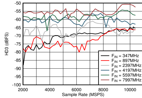
Figure 5-38. DES Mode: HD3 vs Sample Rate and Input Frequency
