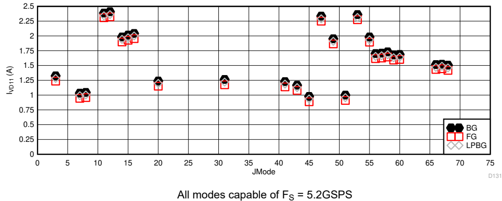
Figure 5-115. Dual Channel Mode: I_{VD11} vs JMODE at 5.2GSPS
