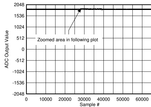
Figure 5-144. Background Calibration Core Transition (DC Signal)
