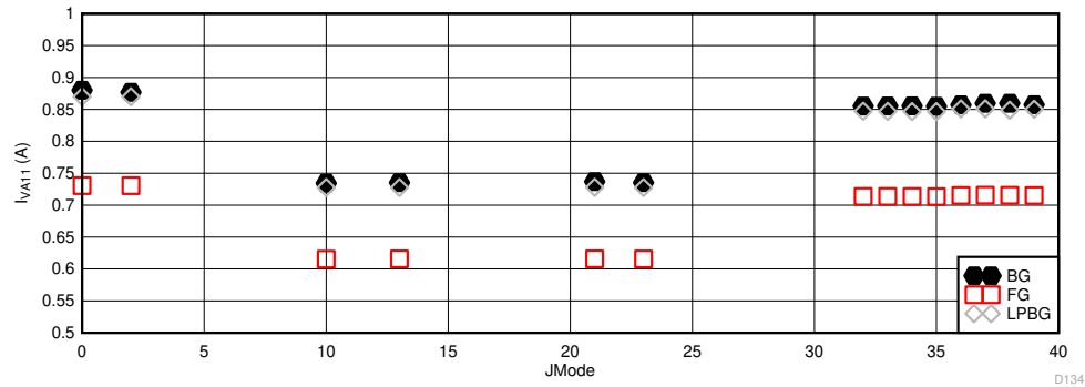
Figure 5-118. Other Modes with Lower Maximum F_S : I_{VA11} vs JMODE
