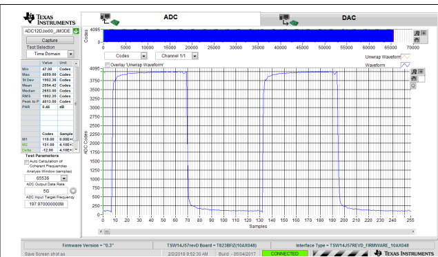
Figure 7-7. 40-MHz, Square-Wave Time Domain for 5-GSPS, Single-Channel Oscilloscope
