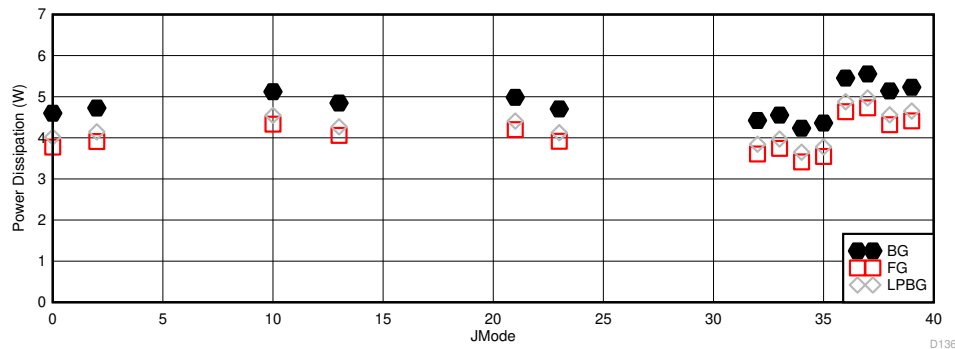
Figure 5-119. Other Modes with Lower Maximum F_S : I_{VD11} vs JMODE
