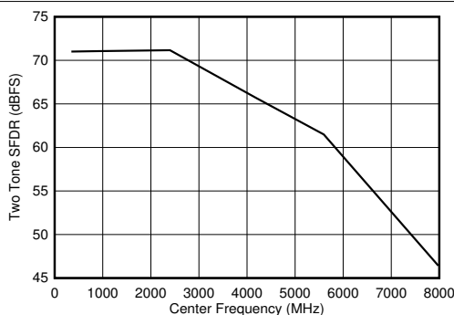
Figure 5-107. Dual Channel Mode: Two Tone SFDR vs Input Frequency
