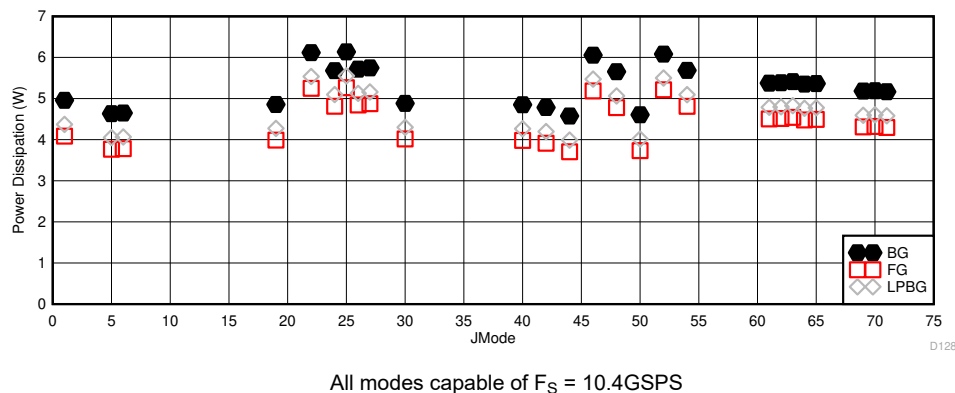
Figure 5-112. DES Mode: Power Dissipation vs JMODE at 10.4GSPS
