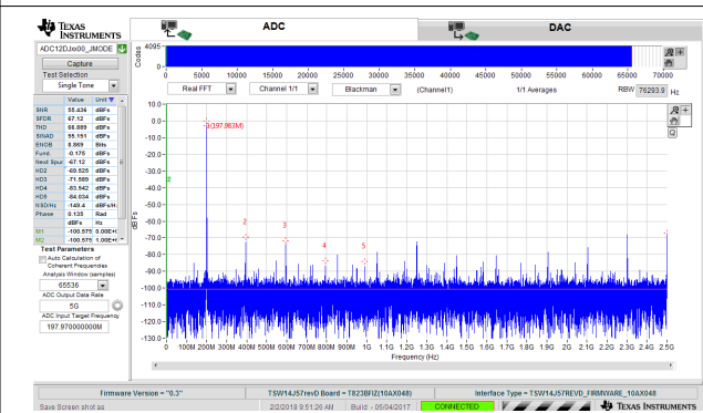
Figure 7-9. 200-MHz, Sine-Wave Frequency Domain (FFT) for 5-GSPS, Single-Channel Oscilloscope
