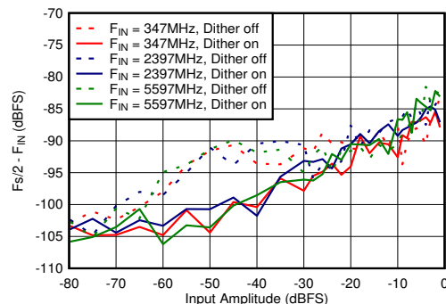
Figure 5-80. Dual Channel Mode: \text{Fs}/2 - F_{\text{IN}} vs Input Amplitude and Dither
