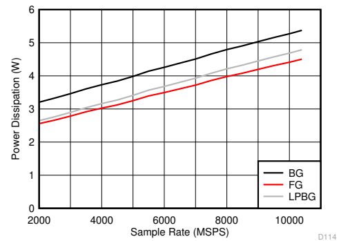
Figure 5-128. DES Mode: Power Dissipation vs Sample Rate
