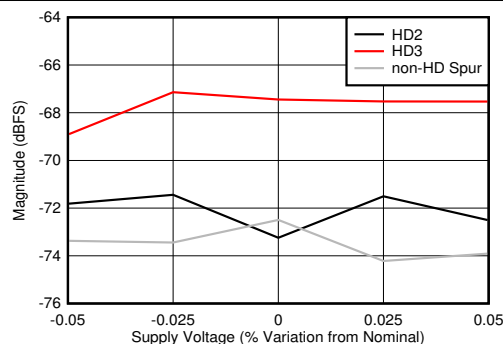
Figure 5-94. DES Mode: HD2, HD3 and Worst non-HD Spur vs Supply Voltage
