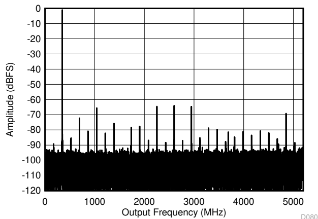
Figure 5-5. DES Mode: Single Tone FFT at 347 MHz
