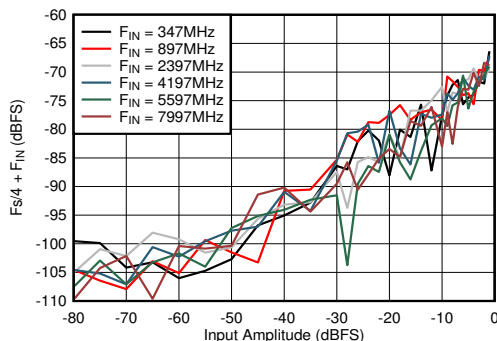
Figure 5-67. DES Mode: F_s/4 + F_{\text{IN}} vs Input Amplitude and Frequency
