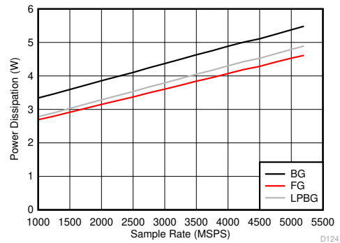
Figure 5-140. Dual Channel Mode: Power Dissipation vs Sample Rate
