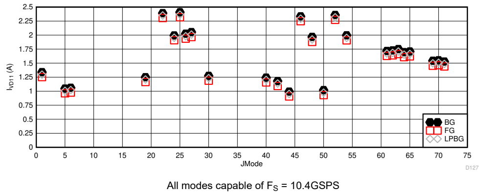
Figure 5-111. DES Mode: I_{VD11} vs JMODE at 10.4GSPS
