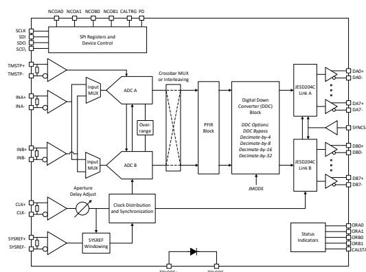
ADC12DJ5200RF Block Diagram
