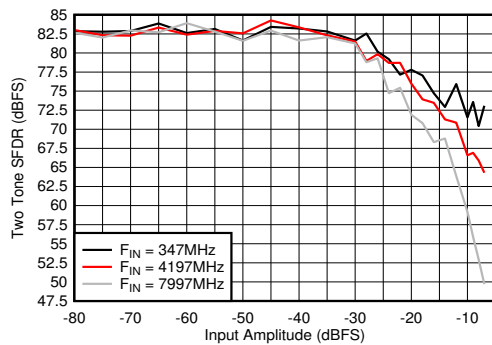
Figure 5-103. DES Mode: Two Tone SFDR vs Input Amplitude
