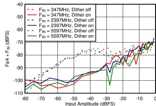
Figure 5-66. DES Mode: \text{Fs}/2 - F_{\text{IN}} vs Input Amplitude and Dither
