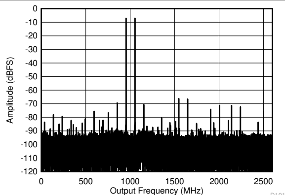
Figure 5-26. Dual Channel Mode: Two Tone FFT at 4197 MHz
