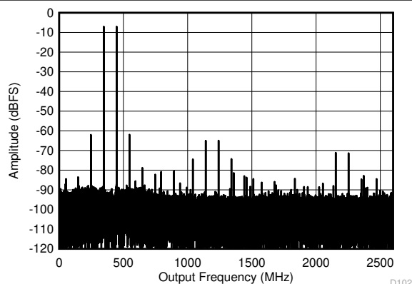
Figure 5-25. Dual Channel Mode: Two Tone FFT at 2397 MHz
