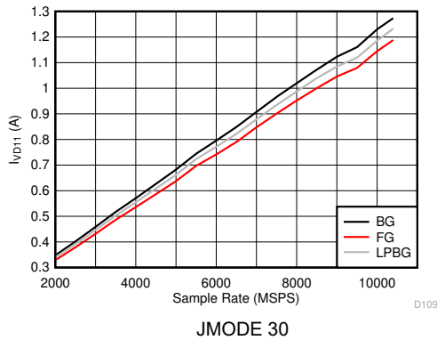
Figure 5-125. DES Mode: I_{VD11} vs Sample Rate
