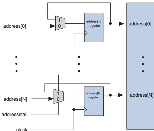
Figure 3-2. Address Clock Enable
