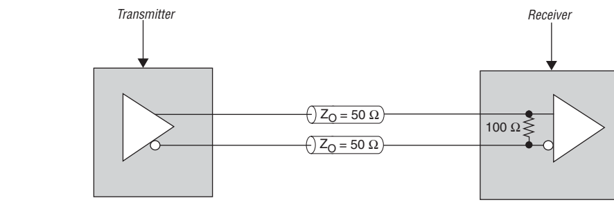
Figure 6-22. Differential Input OCT
