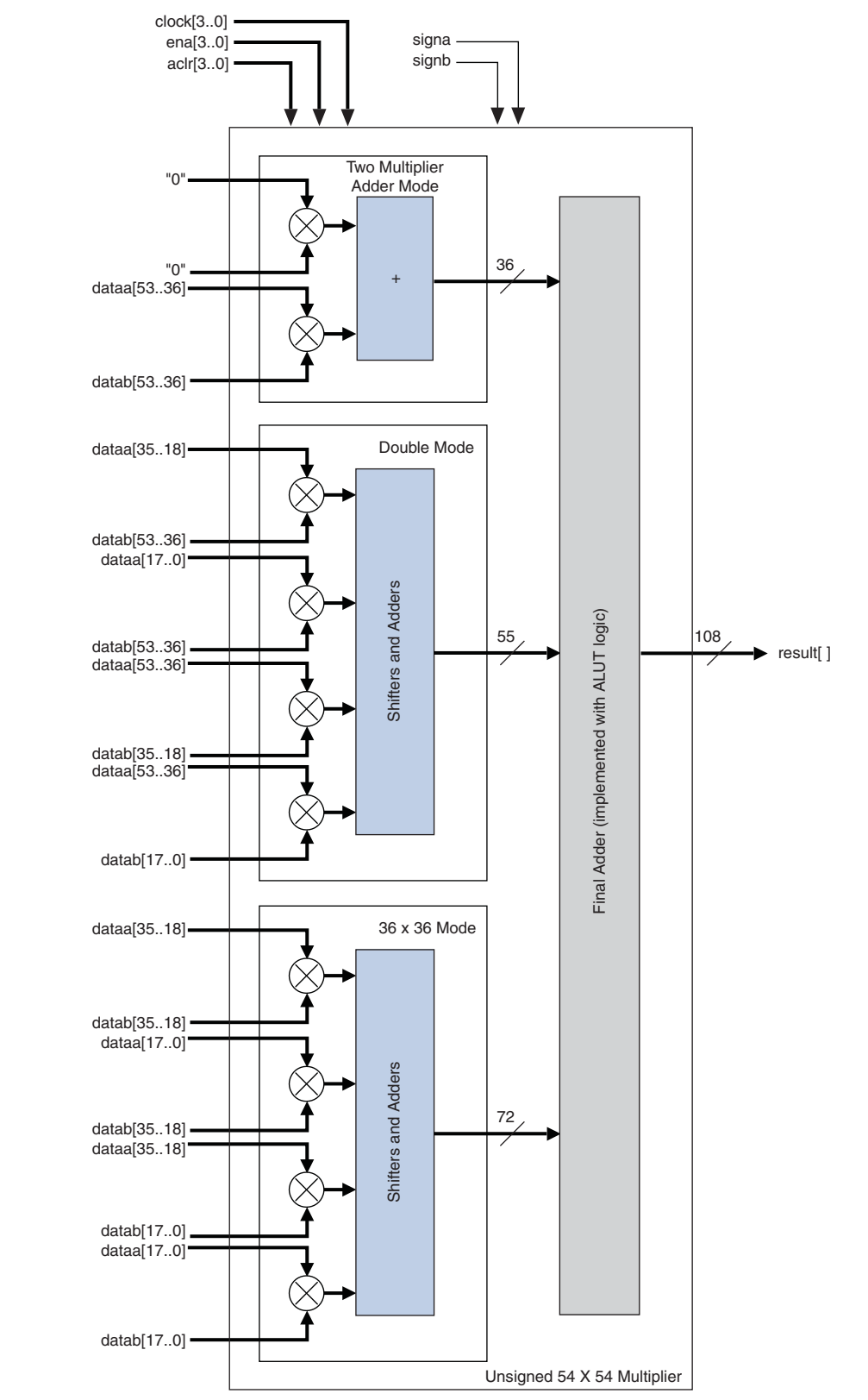
Figure 4-13. Unsigned 54 \times 54 Multiplier for a Half-DSP Block
