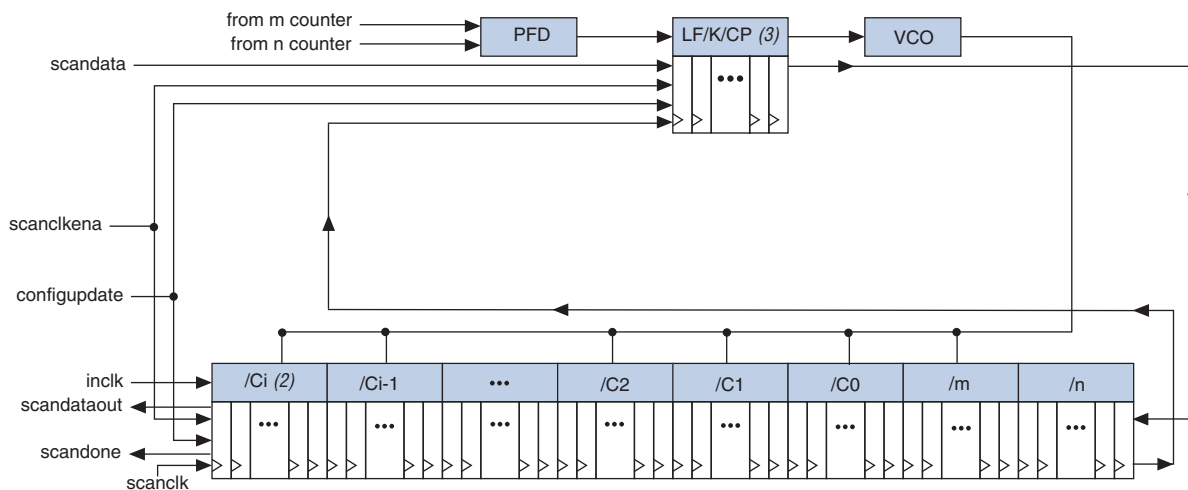
Figure 5-39. PLL Reconfiguration Scan Chain (1)
