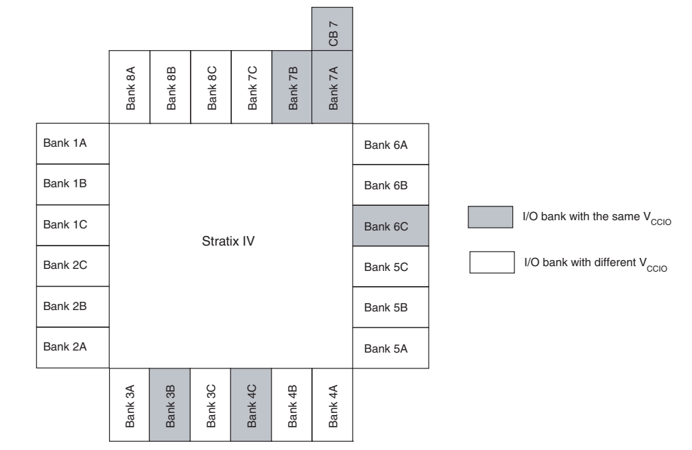
Figure 6-23. Example of Calibrating Multiple I/O Banks with One Shared OCT Calibration Block
