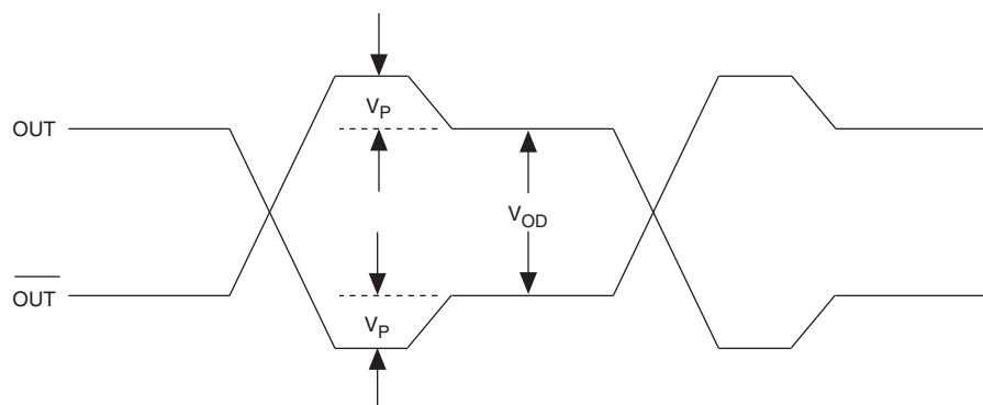
Figure 8-9. Programmable Pre-Emphasis (1)
