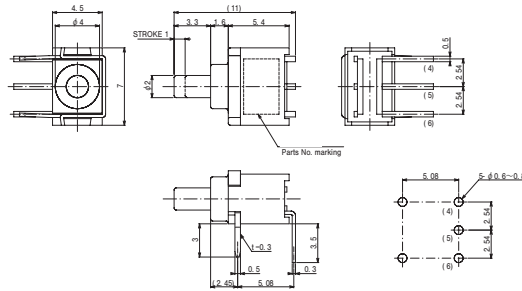
(Top view) PC Hole Layouts
