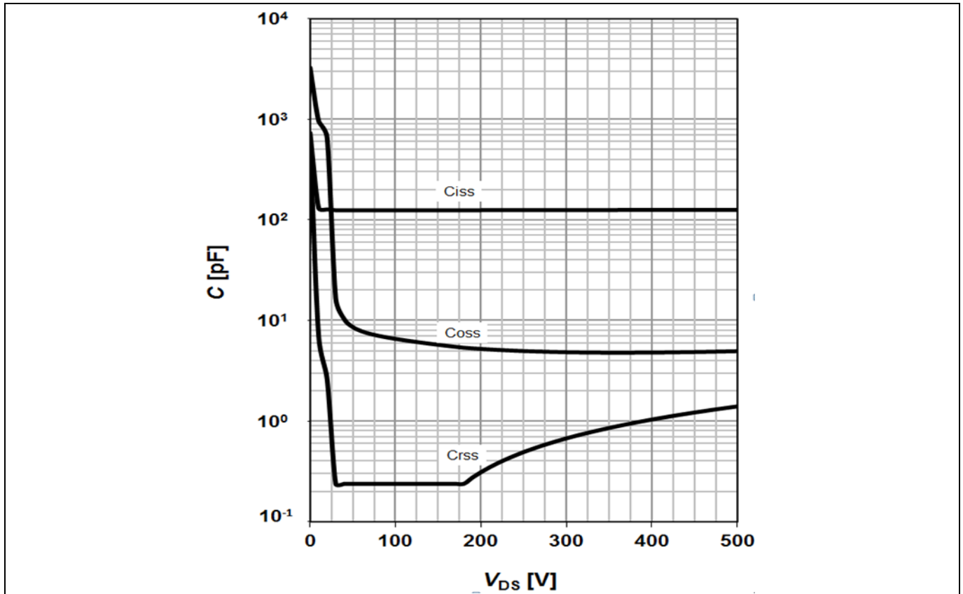
Figure 24 Typical CoolMOS™ capacitances of ICE5QR2280BG ( C=f(V_{DS}); V_{GS}=0 V; f=250 kHz)
