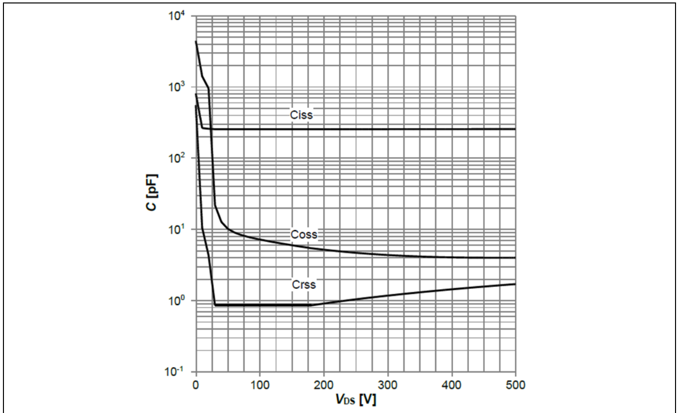
Figure 25 Typical CoolMOS™ capacitances of ICE5QR1680BG ( C=f(V_{DS}); V_{GS}=0 V; f=250 kHz)
