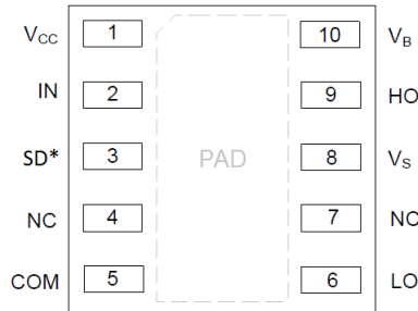
W-DFN3030-10 (Type TH)
