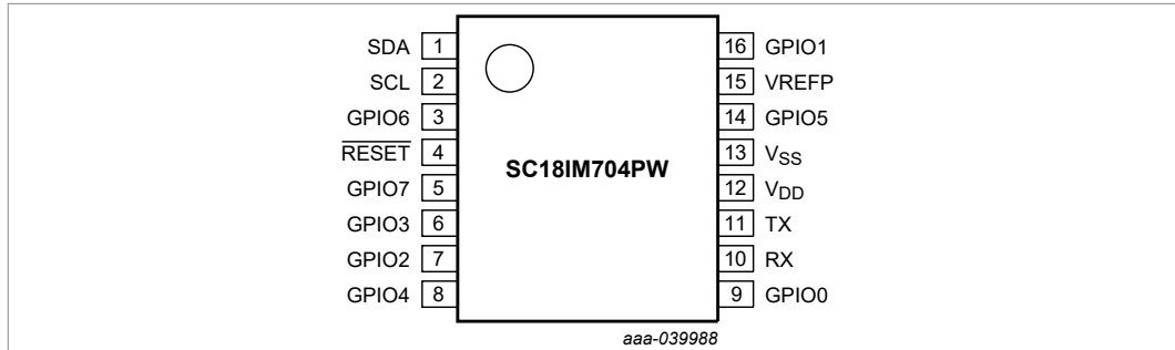
Figure 2. Pin configuration for TSSOP16
