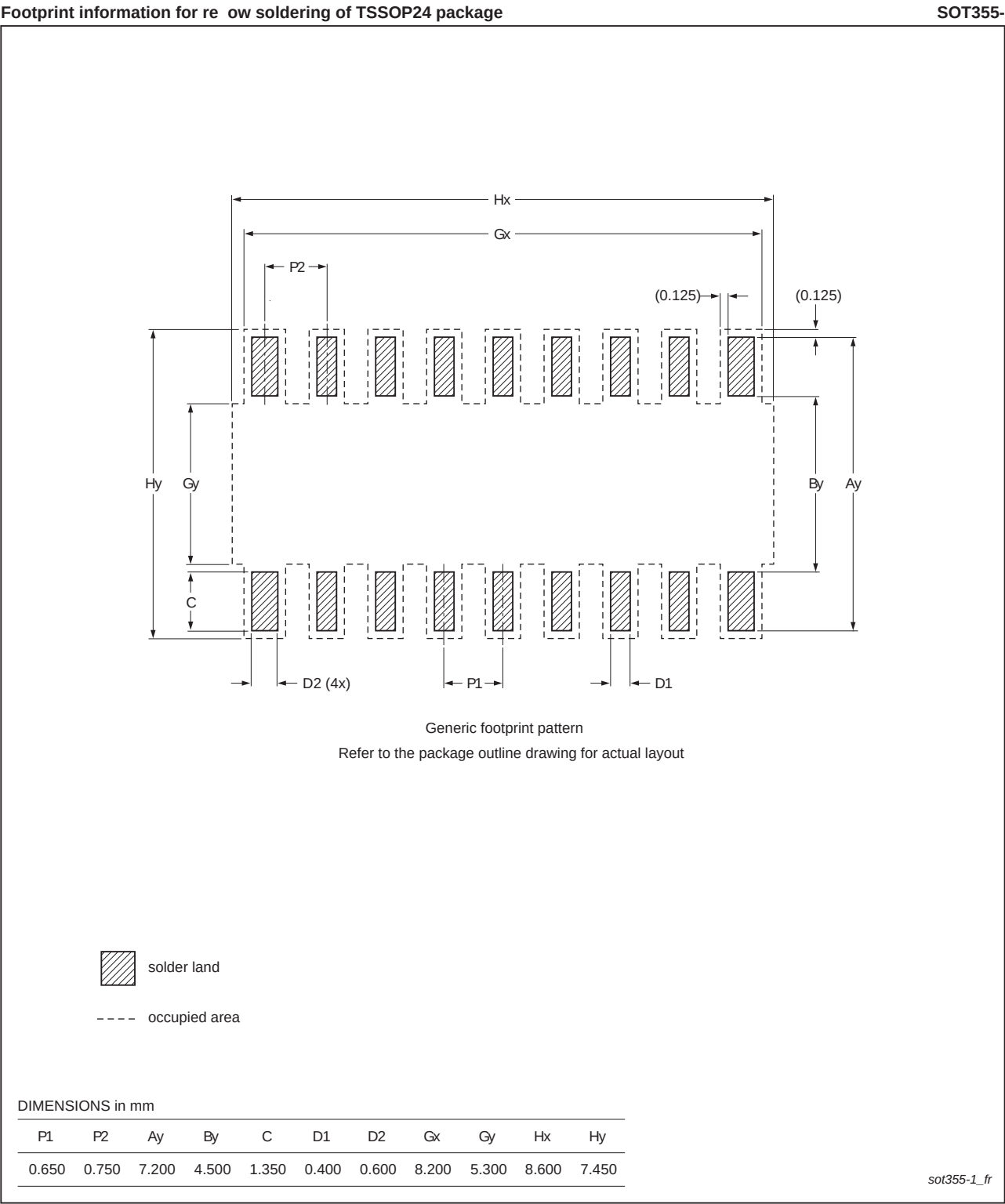
Fig 40. Reflow soldering of the TSSOP24 package
