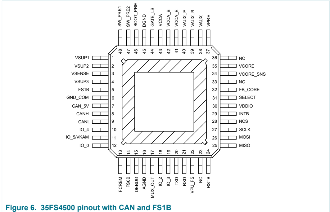
Figure 6. 35FS4500 pinout with CAN and FS1B
