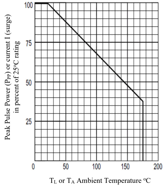
FIG. 4 Derating Curve
