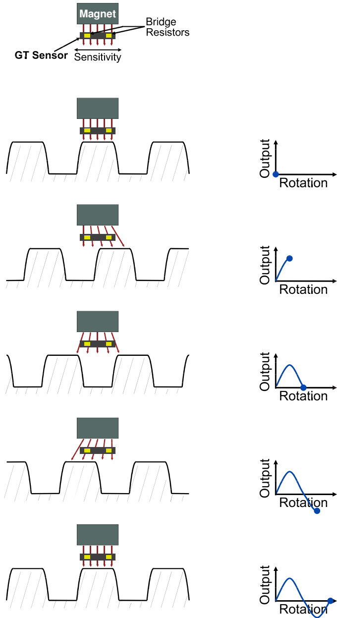
Figure 3. ABL00x output vs. gear rotation.
