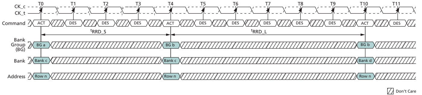
Figure 113: t_{RRD} Timing
