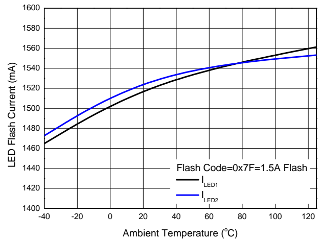
LED Flash Current vs. Temperature
