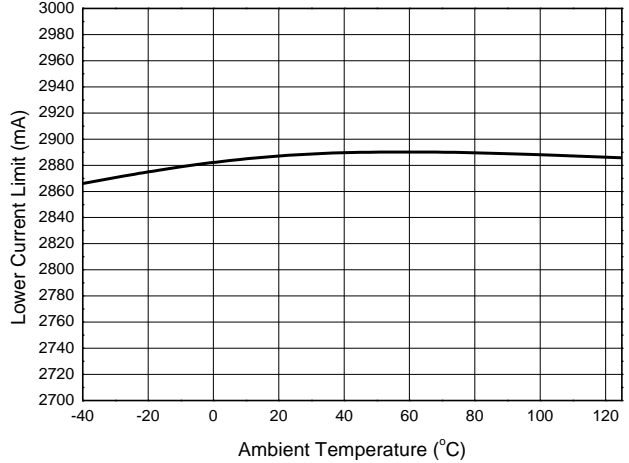
Inductor Current Limit 2 vs. Temperature
