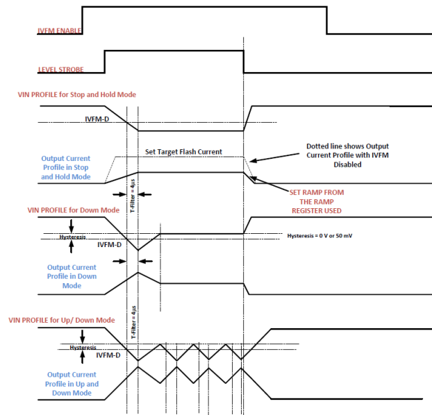
Figure 5. IVFM Modes
