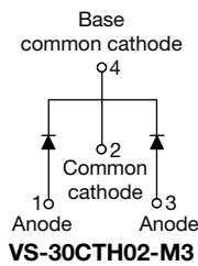
TO-220AB 3L
