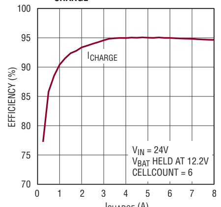
Lead-Acid Charging Efficiency vs I_{CHARGE}
