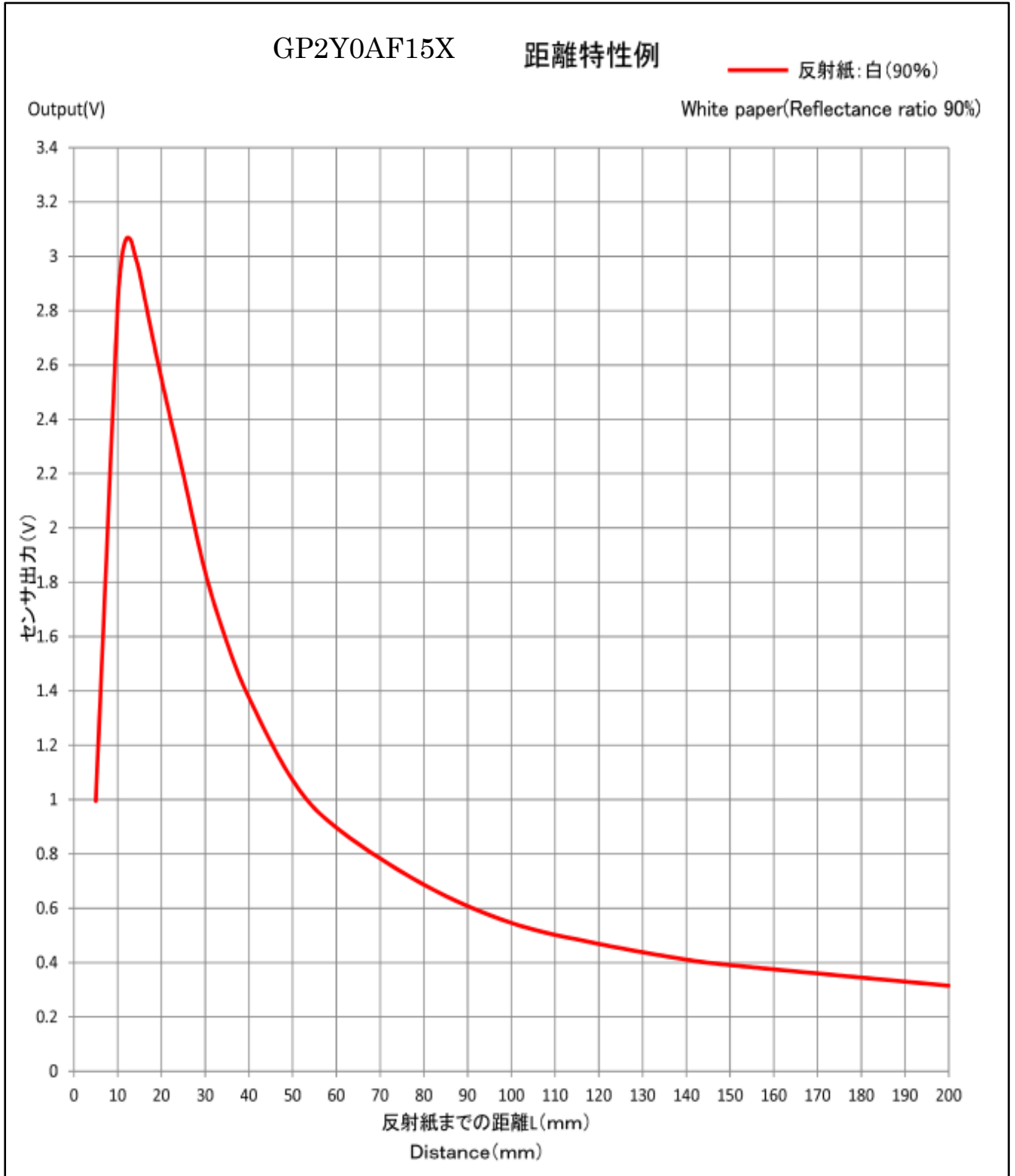
GP2Y0AF15X Example of output distance characteristics
