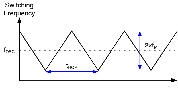
Figure 35. Frequency Hopping
